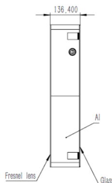
Module Dimensions and mounting locations(mm)
