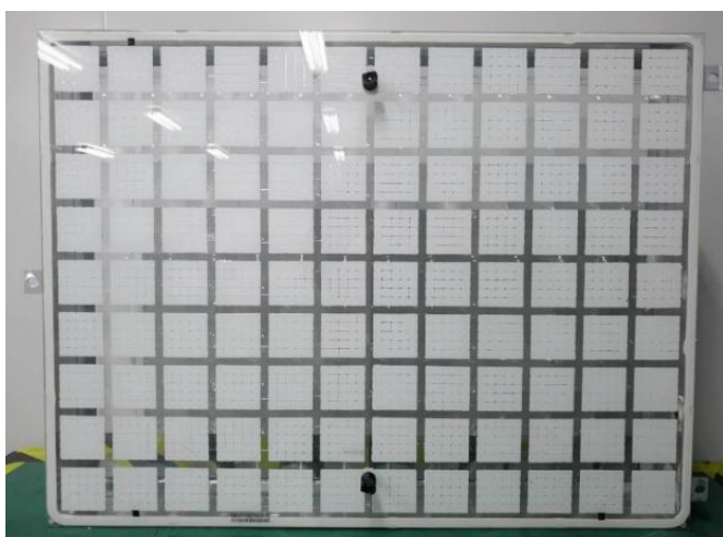
MS-HCPV120W-750X Module physical photos and wire connection
