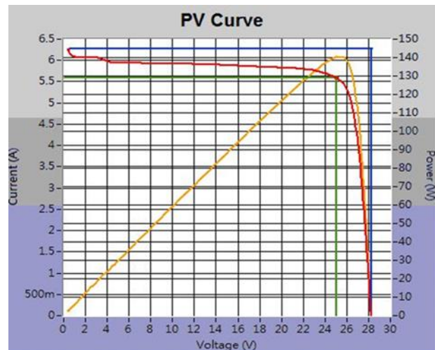
I-V Characteristics of MS-HCPV120-750X
